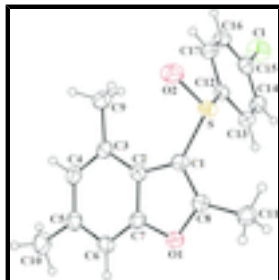
Fig. 1. The molecular structure of the title compound with the atom numbering scheme. Displacement ellipsoids are drawn at the 30% probability level. H atoms are presented as spheres of arbitrary radii.
